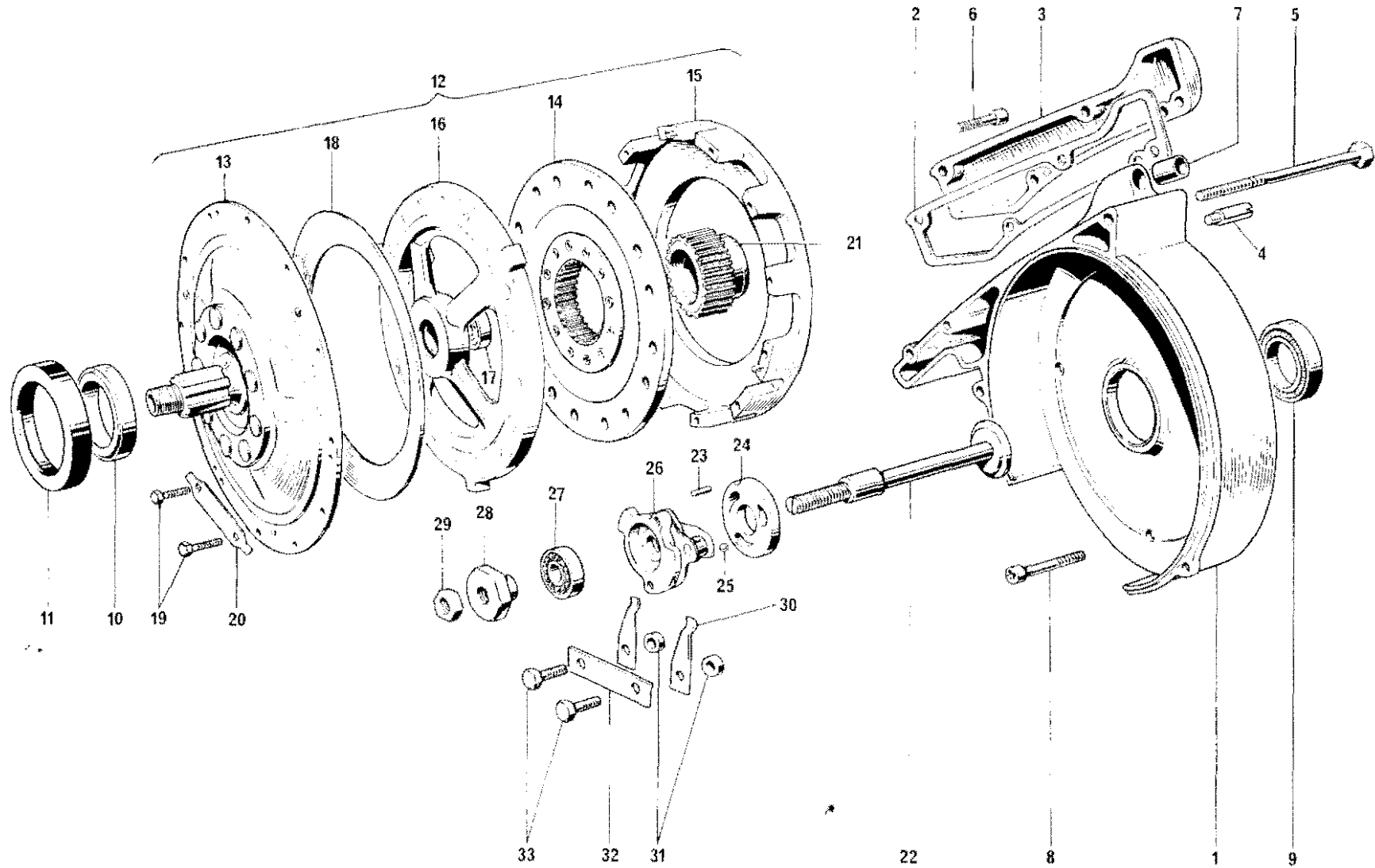
Fig. 11. CLUTCH AND CLUTCH OPERATION
