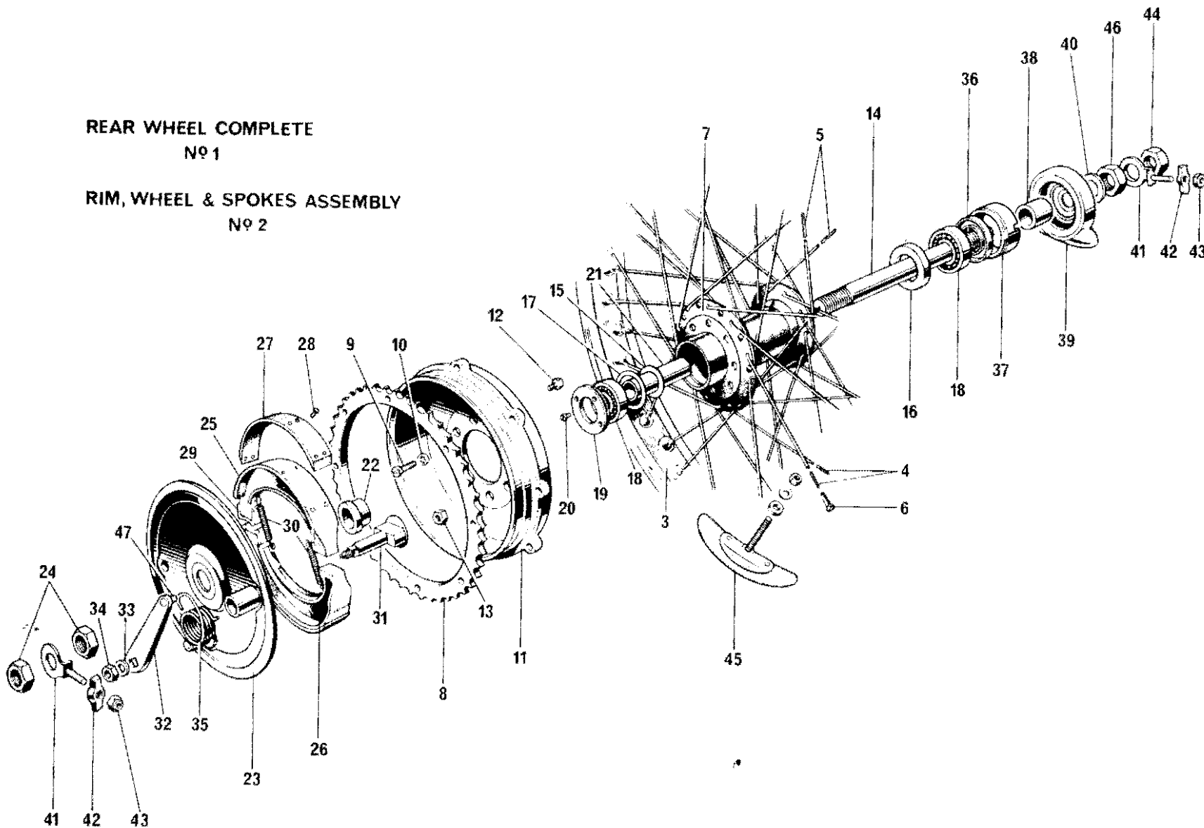
Fig. 21. REAR WHEEL
