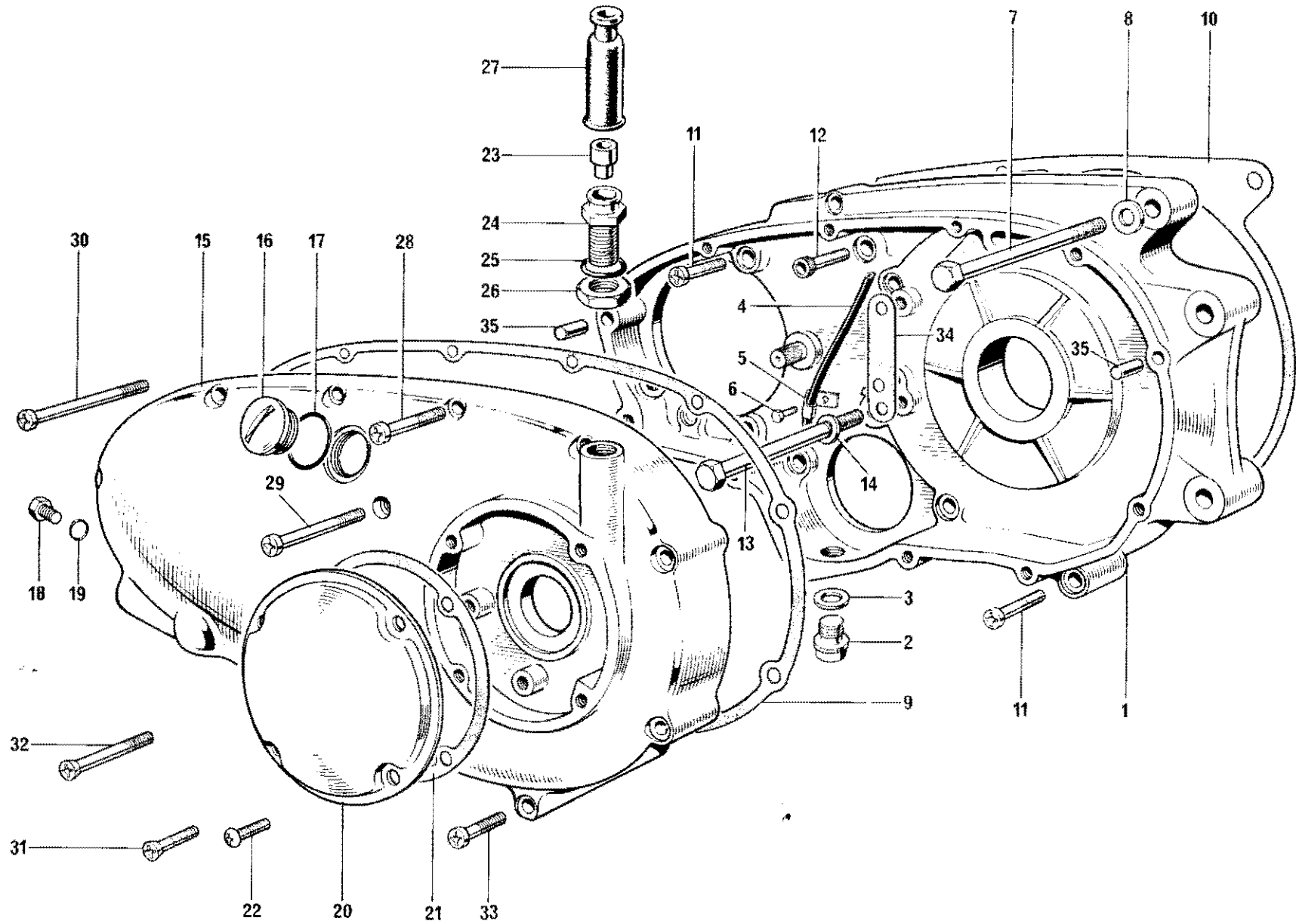
Fig. 12. INNER AND OUTER CHAINCASE
