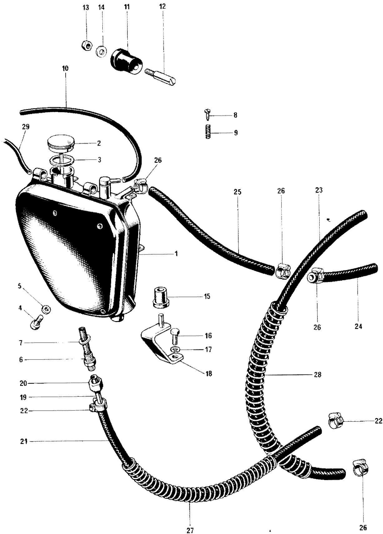
Fig. 24. OIL TANK
