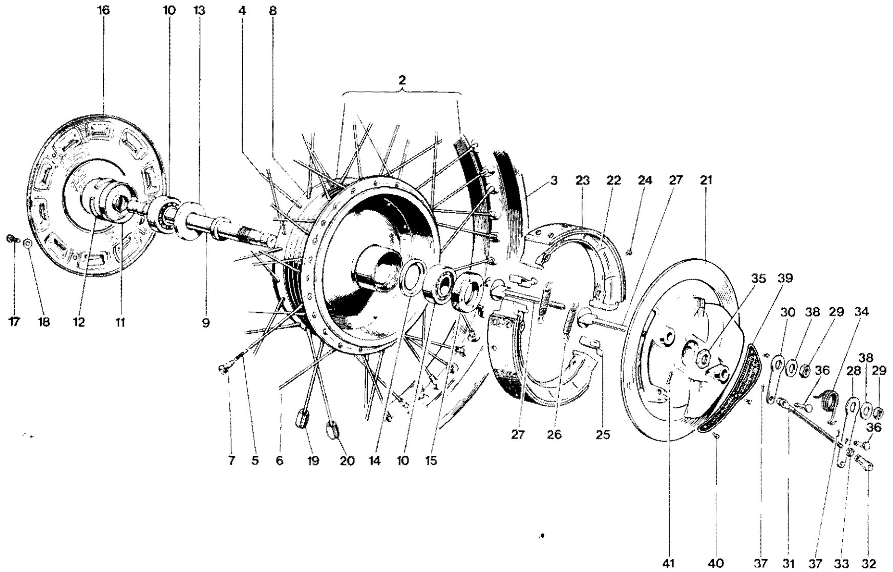
Fig. 20 FRONT WHEEL
