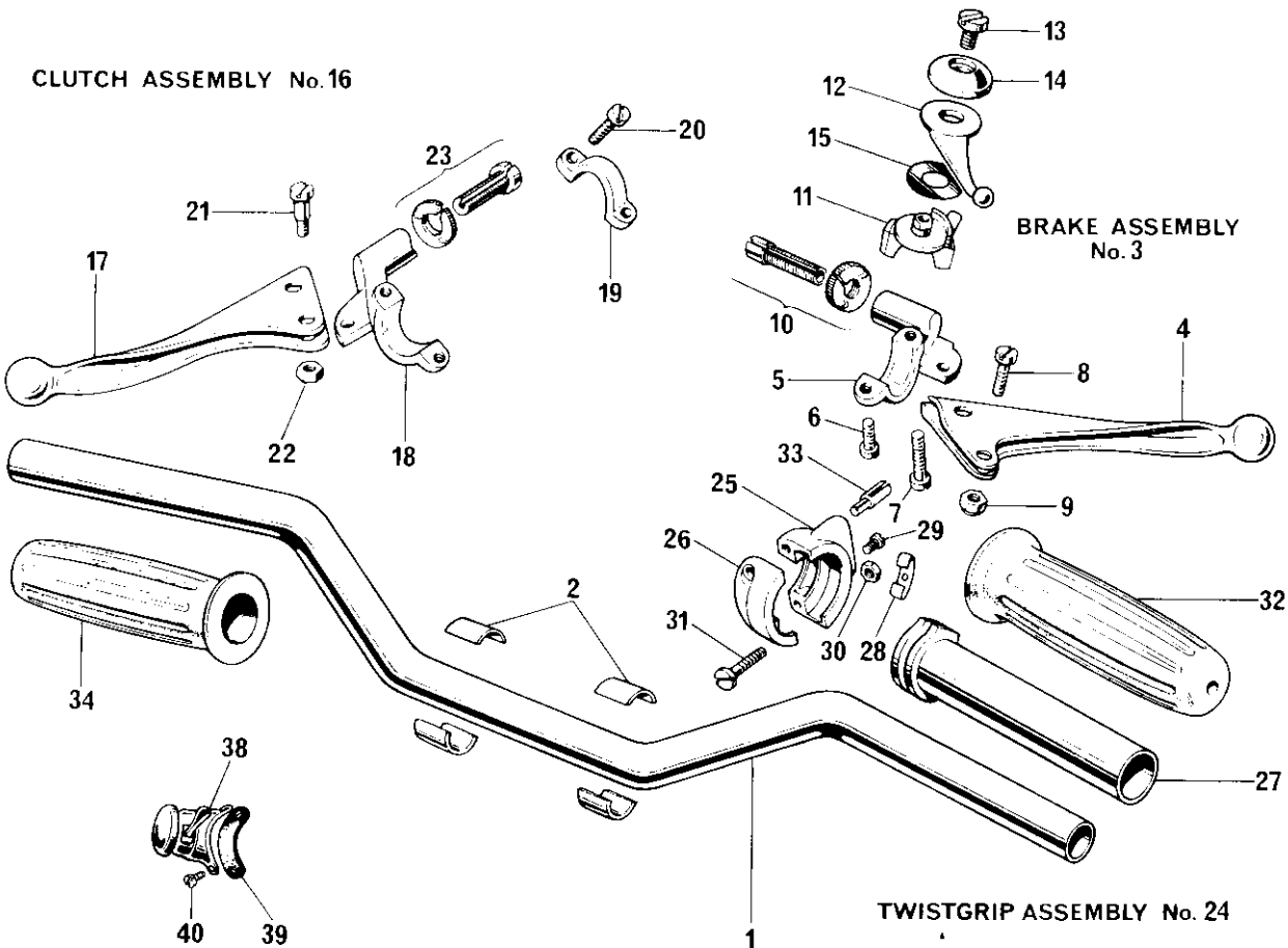
Fig. 28. HANDLEBARS, CONTROLS, BINNACLE AND OIL WARNING LIGHT
